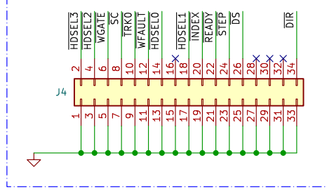
Control cable pin header
