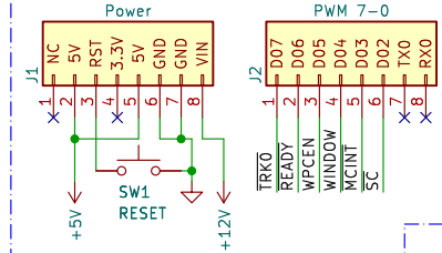
Mega2560 board pin headers
