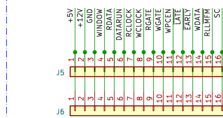
Separator board pin sockets (board orientation-independent)
