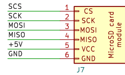
Card adapter pin header
