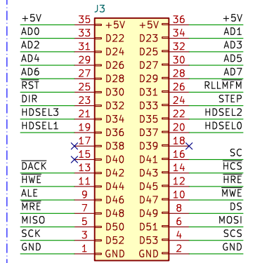
Control cable pin header
