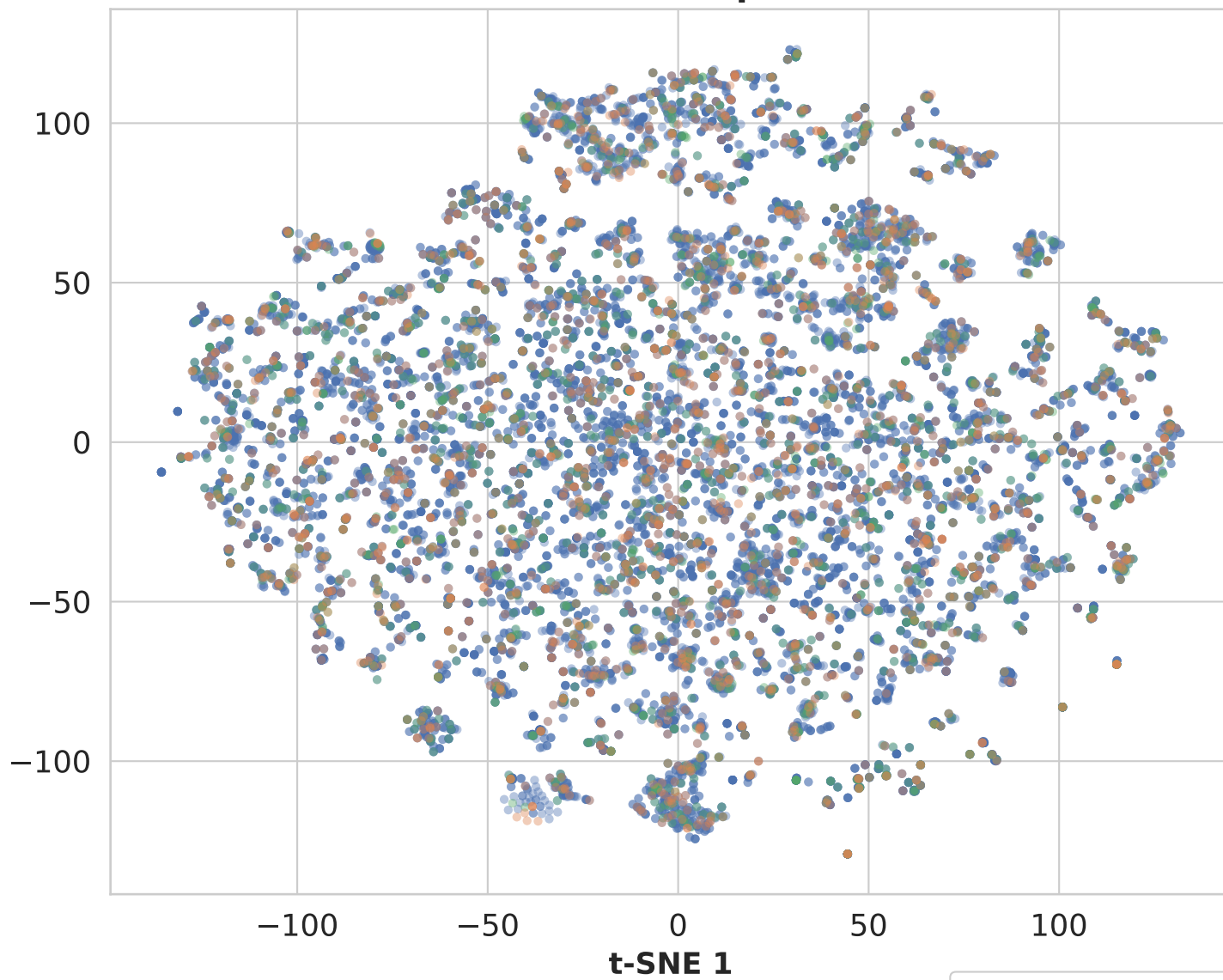
Random Split
