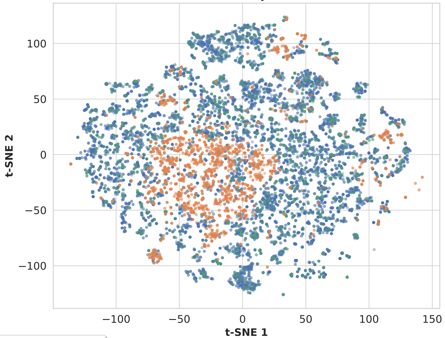
aCSM Split
