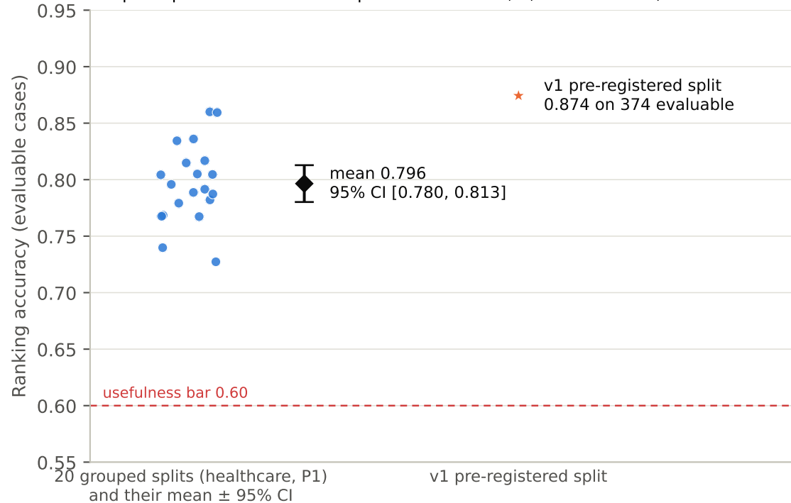
a Split replication — 20 of 20 splits clear the bar; 5,489 evaluable, 573 excluded
