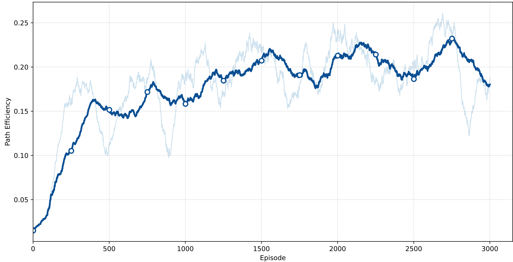
Path Efficiency vs Episode
