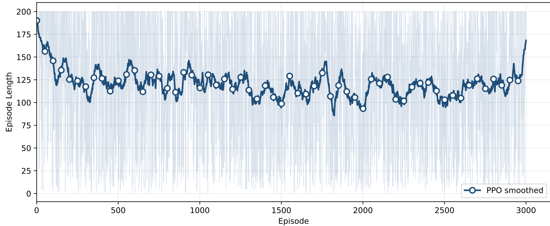
Saved PPO Training Episode Length vs Episode
