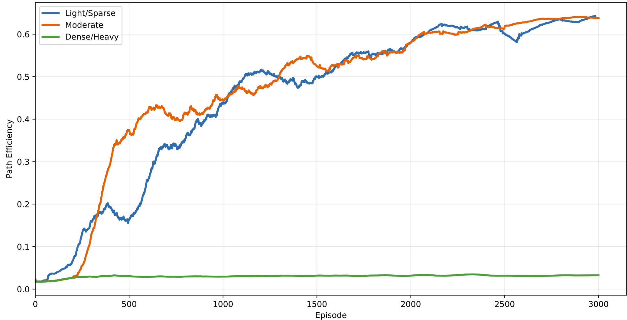
Path Efficiency vs Episode by Fire-Density Map
