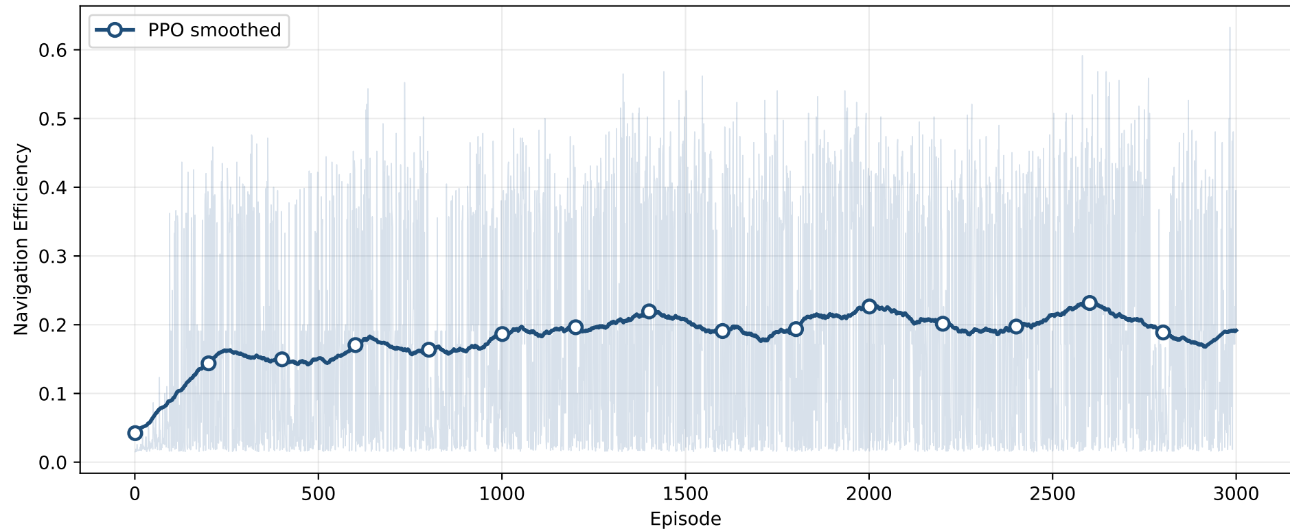
Saved PPO Training Efficiency vs Episode
