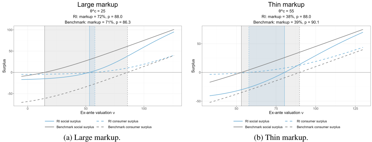
Figure 5: Extensive-margin cutoffs under RI and the optimal-refund benchmark. Panels vary \theta^c at each scheme’s monopoly price.
