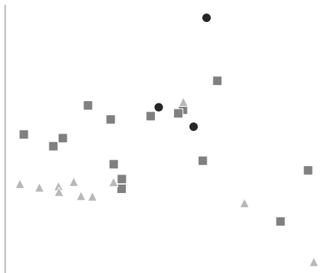
LMV St. Francis basin (n=29, 3 spatial clusters, F_{ST}=+0.018 )
