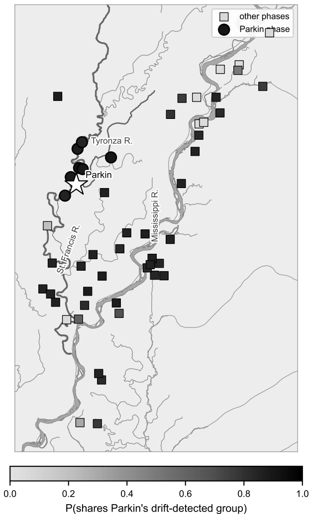
A. Does the Parkin phase pull out of the wider LMV set? (500 river-network drift runs, no boundary imposed)
