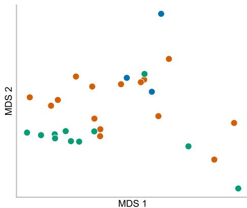
LMV St. Francis basin (n=29, 3 spatial clusters, F_{ST}=+0.018 )
