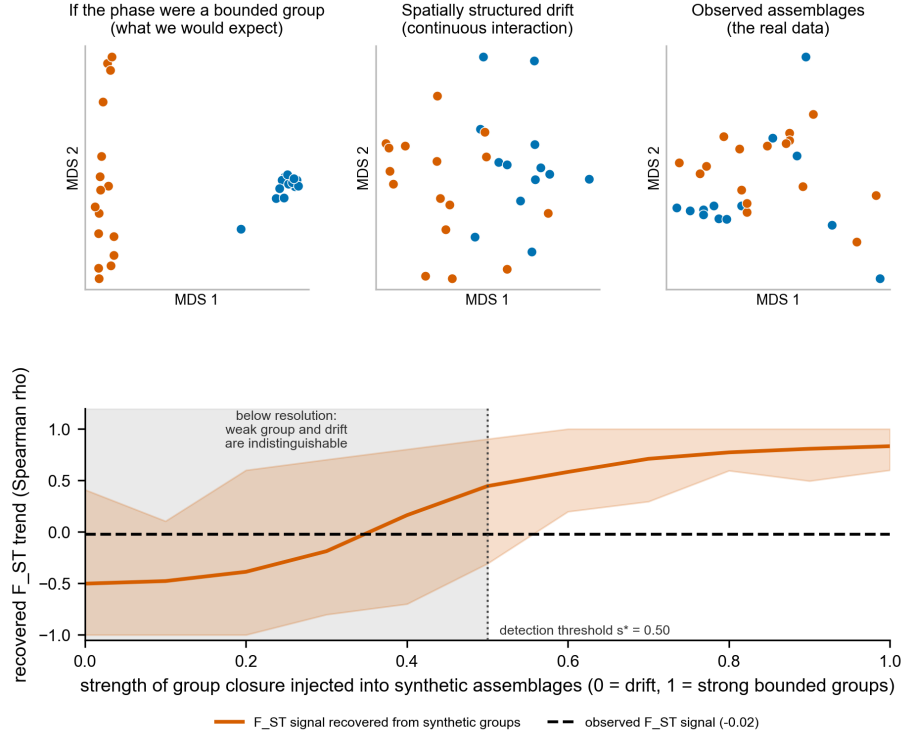
Figure 2. What the test distinguishes, and why the within-basin determination is hard, from synthetic assemblages matched to the record. Top: the basin assemblages in a multidimensional scaling of decorated dissimilarity (points colored by the k=2 spatial split) as they would appear if the Parkin phase were a bounded interaction group (left, sharp clusters), under spatially structured neutral drift (center, a continuous gradient), and as observed (right, a diffuse scatter resembling drift). Bottom: the cultural F_{ST} signal recovered from synthetic assemblages as the strength of injected group closure rises from 0 (drift) to 1 (strong groups), with the s=0 null band shaded behind it. The signal clears the detection threshold only at s^* = 0.5 . The observed value (dashed line) lies in the shaded region below s^* , where a weak group and pure drift are indistinguishable at this record's size and time-averaging. This is why a weak within-basin boundary cannot be excluded.
