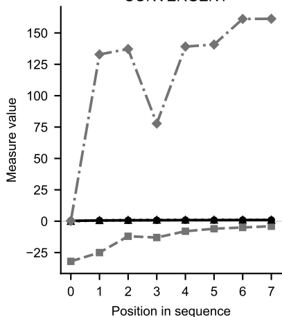
Bounded groups * CONVERGENT
