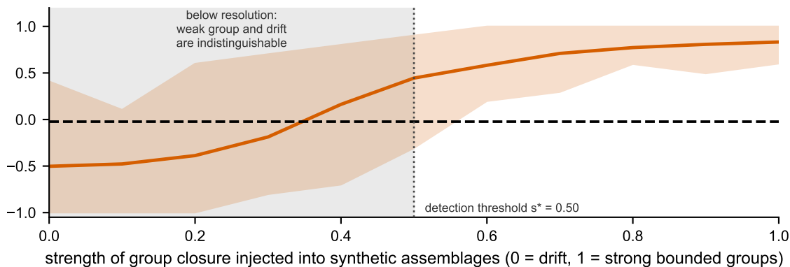
recovered F_{ST} trend (Spearman \rho )
