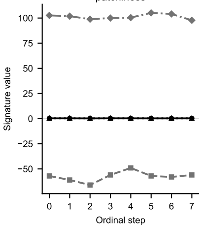
Spatial patchiness
