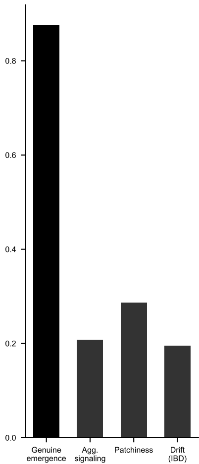
Mean |r| among four signatures
