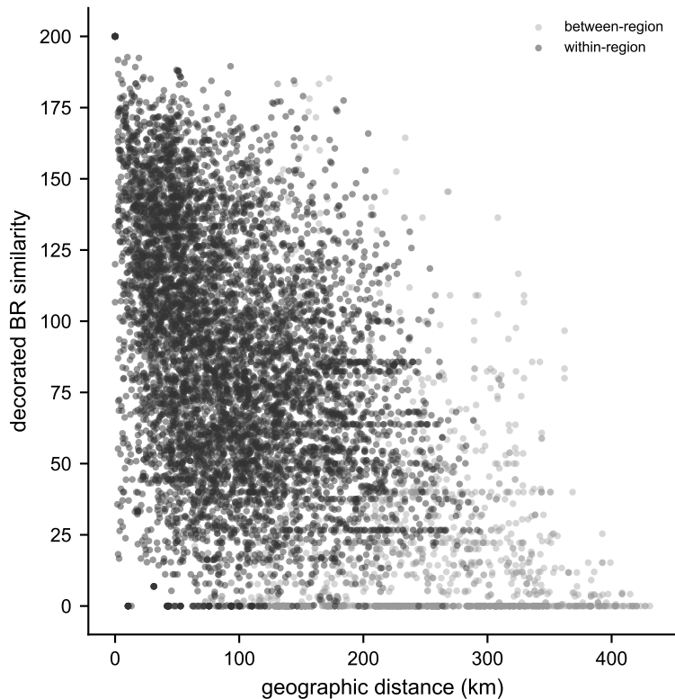
Distance-decay (Mantel r=-0.55 )
