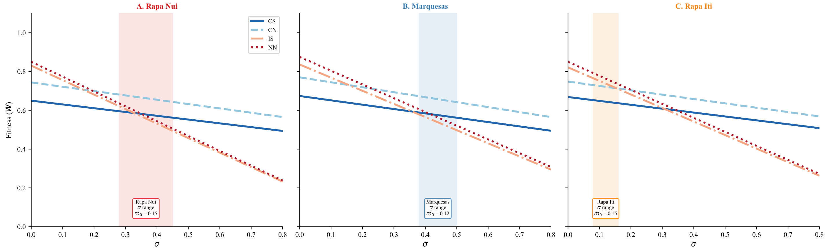
Figure 15. Four-strategy fitness crossover at observed m_0
