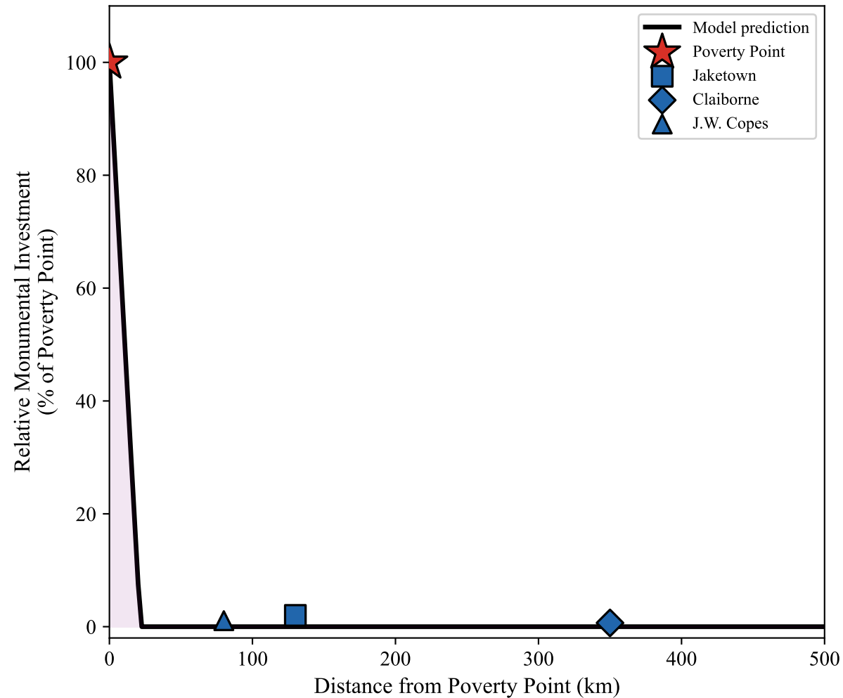
B. Distance-Decay Prediction for Regional Participation
