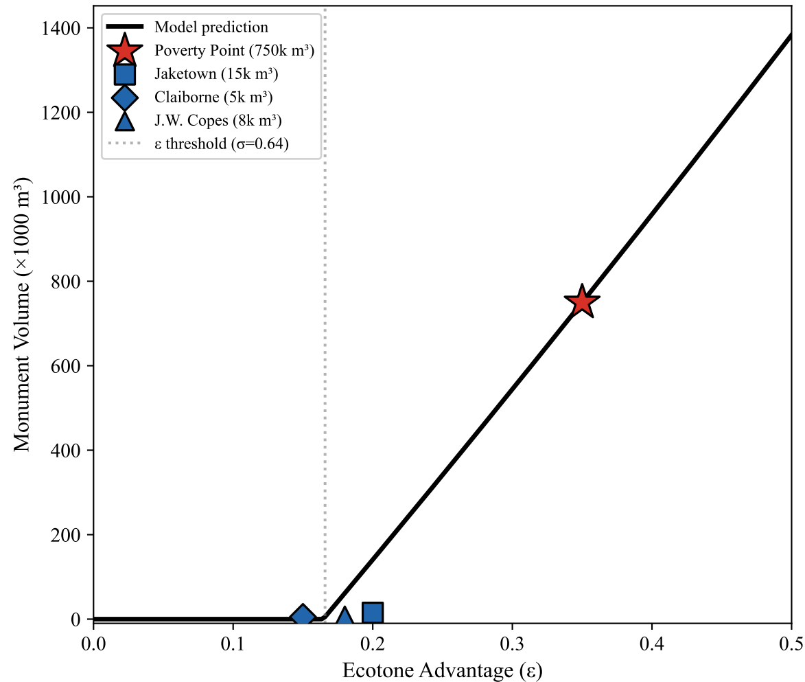
A. Predicted Monument Investment vs. Ecotone Access
