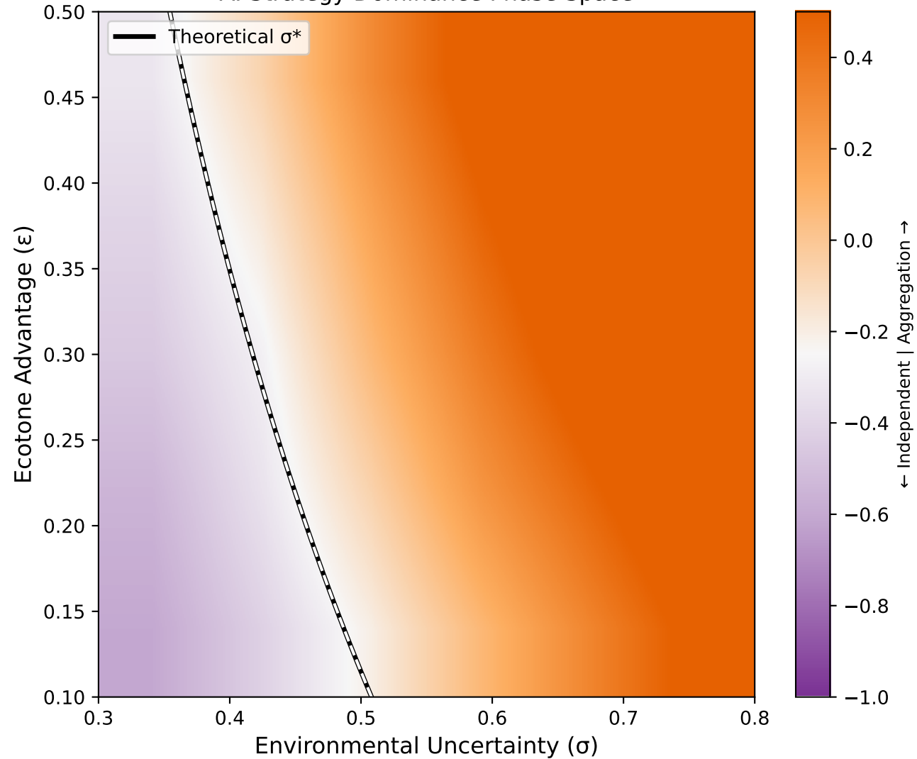
A. Strategy Dominance Phase Space
