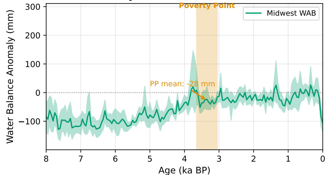
B. Midwest Hydroclimate (Salonen et al. 2025)
