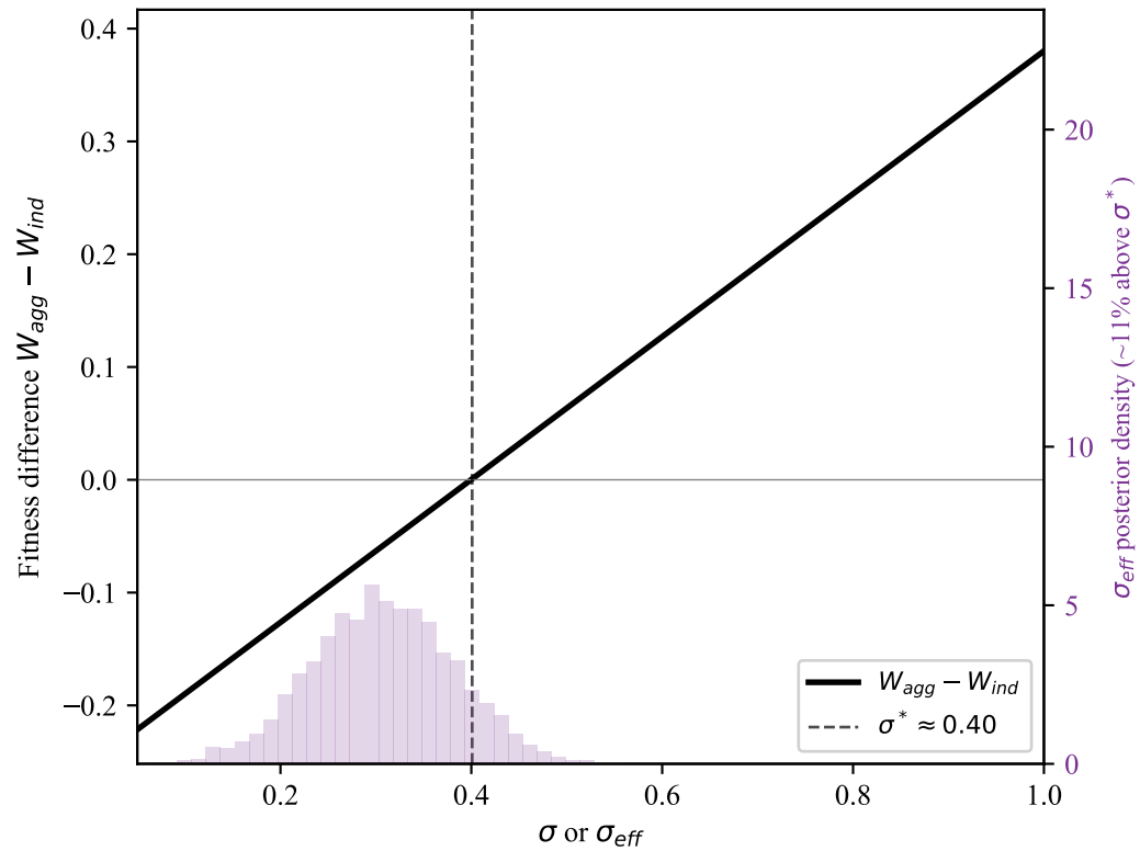
(B) Fitness advantage with \sigma_{eff} posterior
