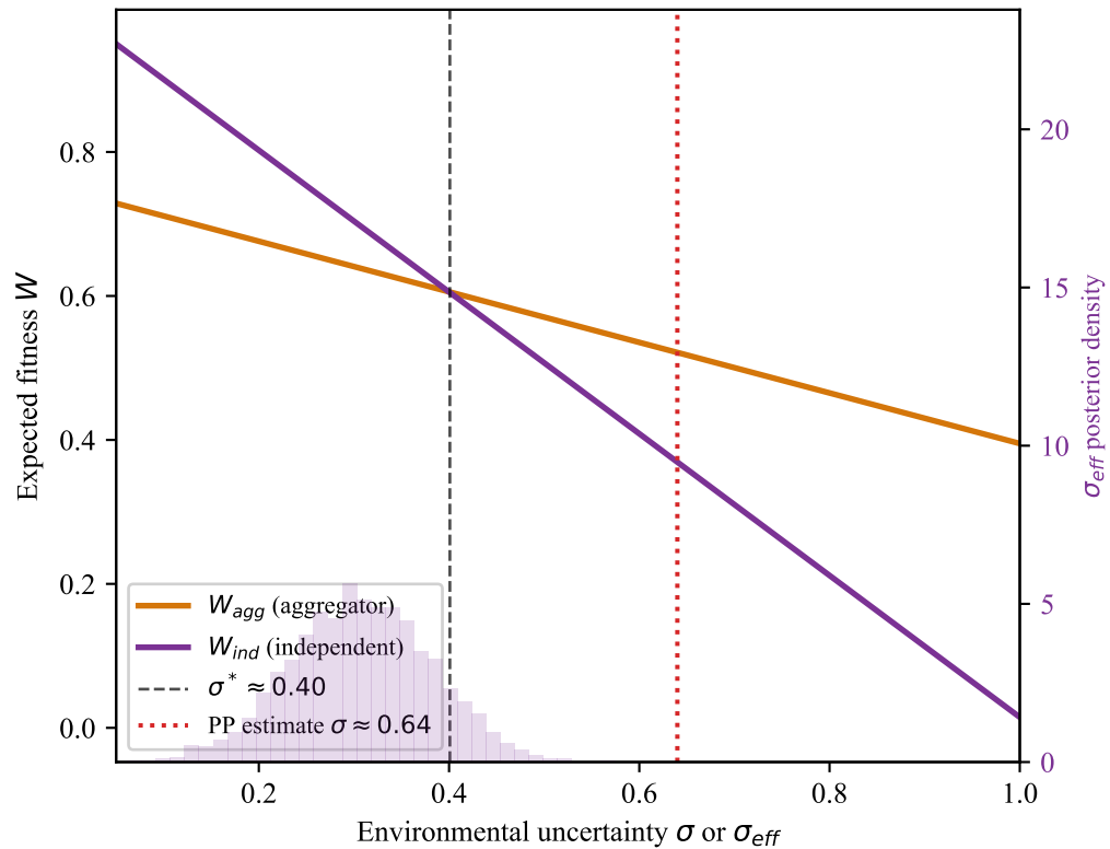
(A) Fitness curves and crossover
