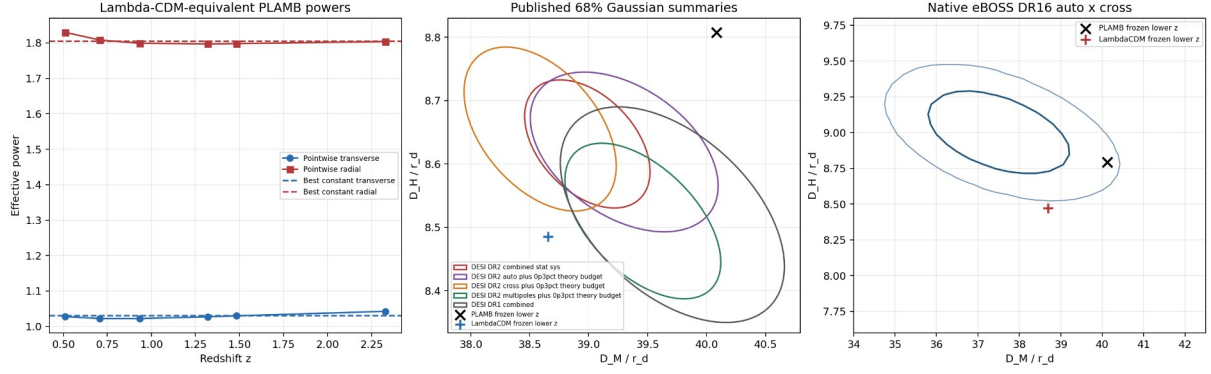
Figure 4. Lambda-CDM-equivalent powers, published DESI Gaussian summaries, and the native eBOSS DR16 auto \times cross likelihood. The same-spectra DR2 multipole control preserves the rejection, whereas the independent eBOSS surface does not.
