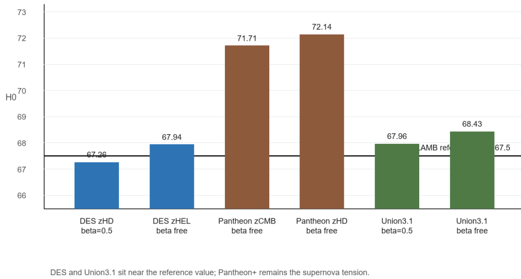
Figure 1. Selected full-covariance raw-MU time-projection results. DES and Union3.1 sit near the PLAMB reference H_0 , while Pantheon+ remains the main tension.
