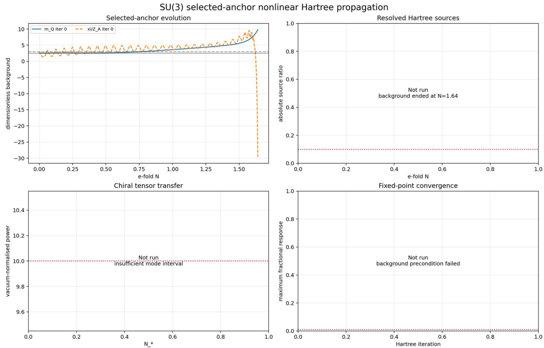
Figure 7. Nonlinear propagation of the selected m_Q=2.5 anchor. The background terminates at N=1.64 ; the empty transfer and Hartree panels record failed physical preconditions rather than missing computation.
