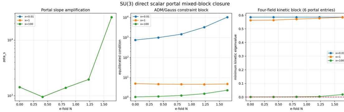
Figure 8. Scalar portal mixed-block closure. The direct field-strength derivative and independent Hessian assembly agree while the reduced kinetic sector remains positive.
