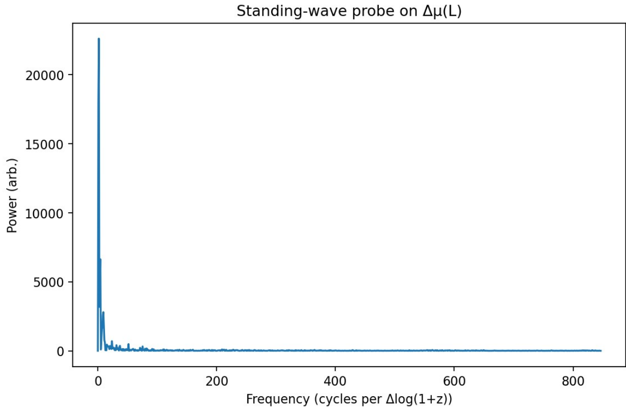
Fig. 6 — Standing-wave probe on \Delta\mu(L) . The near-zero-frequency dominance is consistent with a chirp rather than a strong stationary line.
