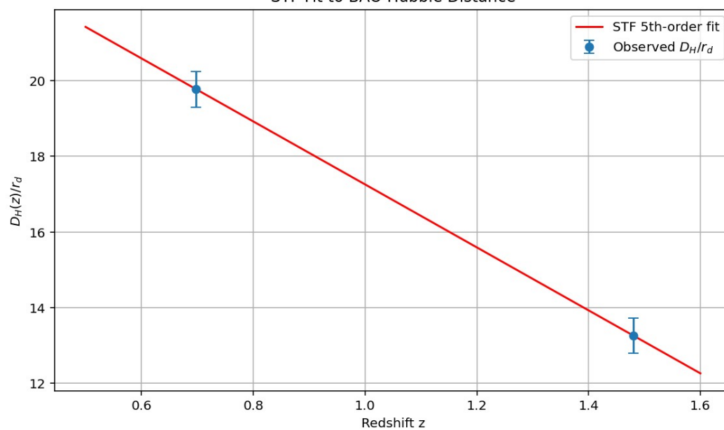
STF Fit to BAO Hubble Distance
