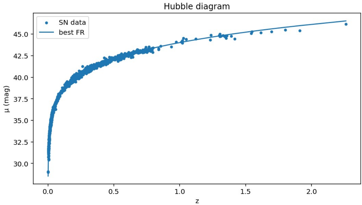
Figure: Hubble diagram, FR ( \Omega\Lambda=0 fixed).
