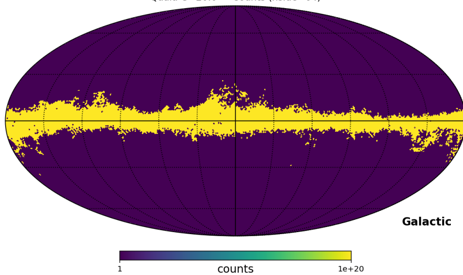
Quiaia G<20.0 — Counts (nside=64)
