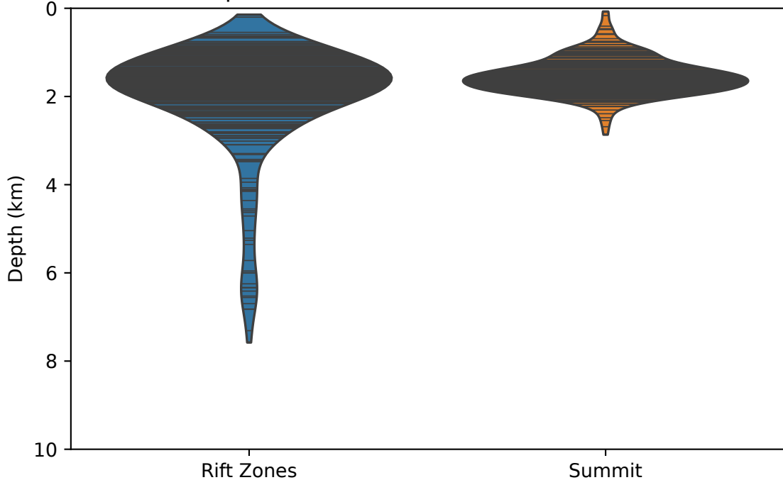
Depth Distribution: Rift Zones vs Summit
