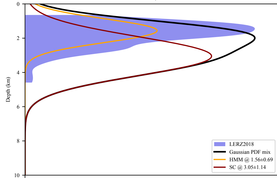
HMM=30% | SC=70%
