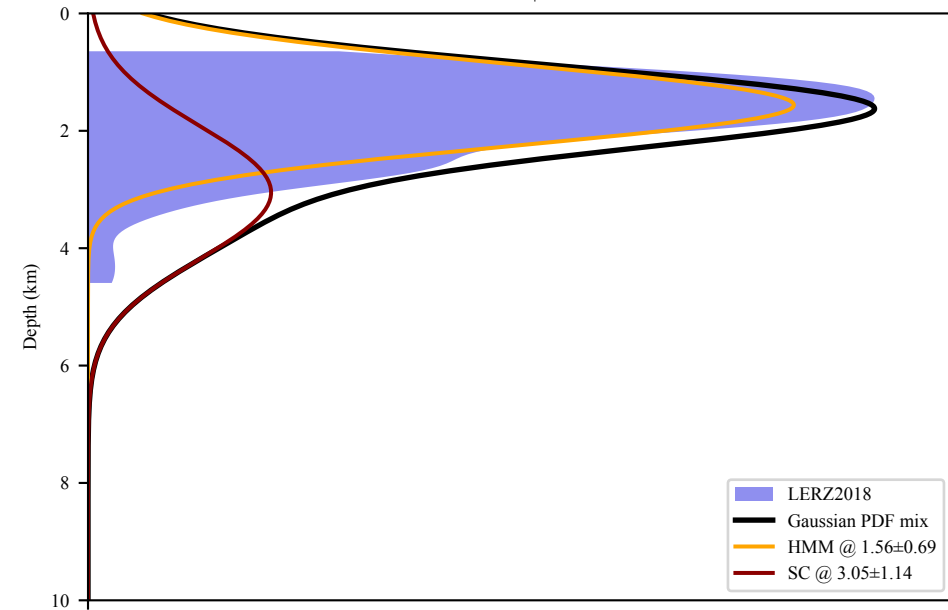
HMM=70% | SC=30%
