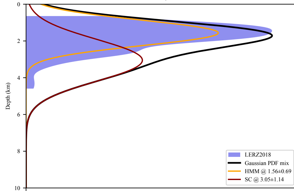
HMM=50% | SC=50%
