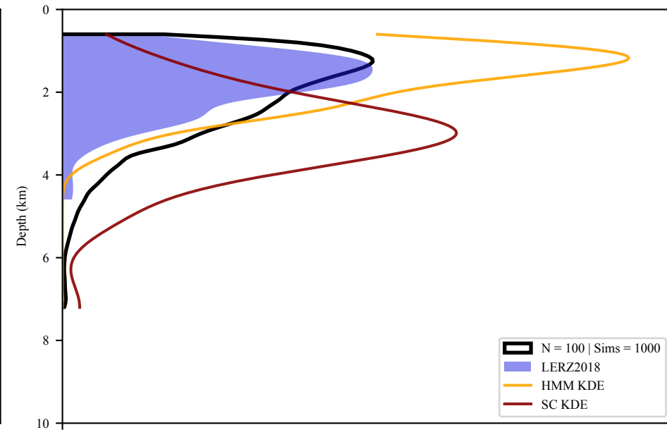
HMM=70%
