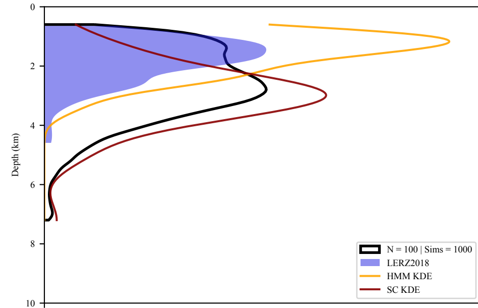
HMM=30%
