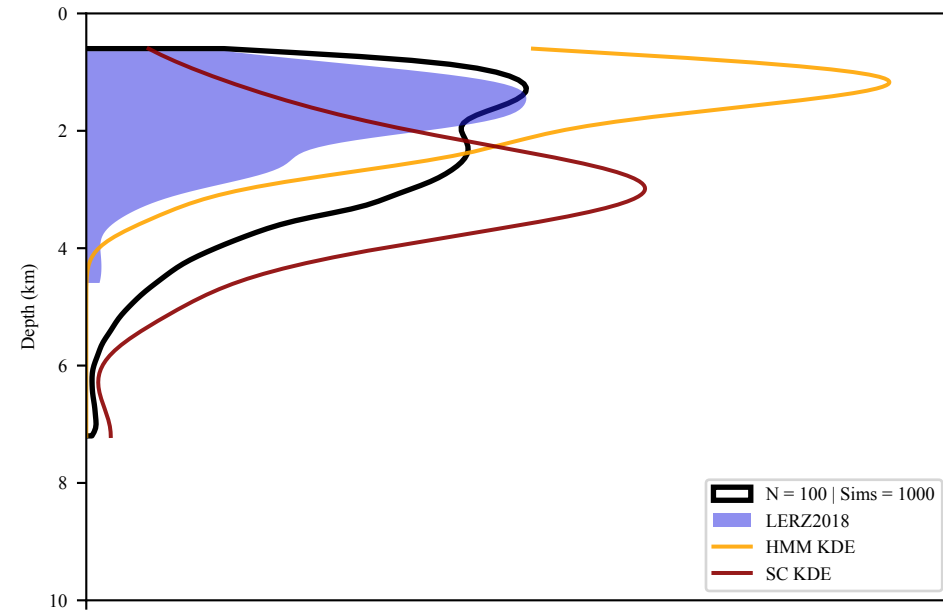
HMM=50%
