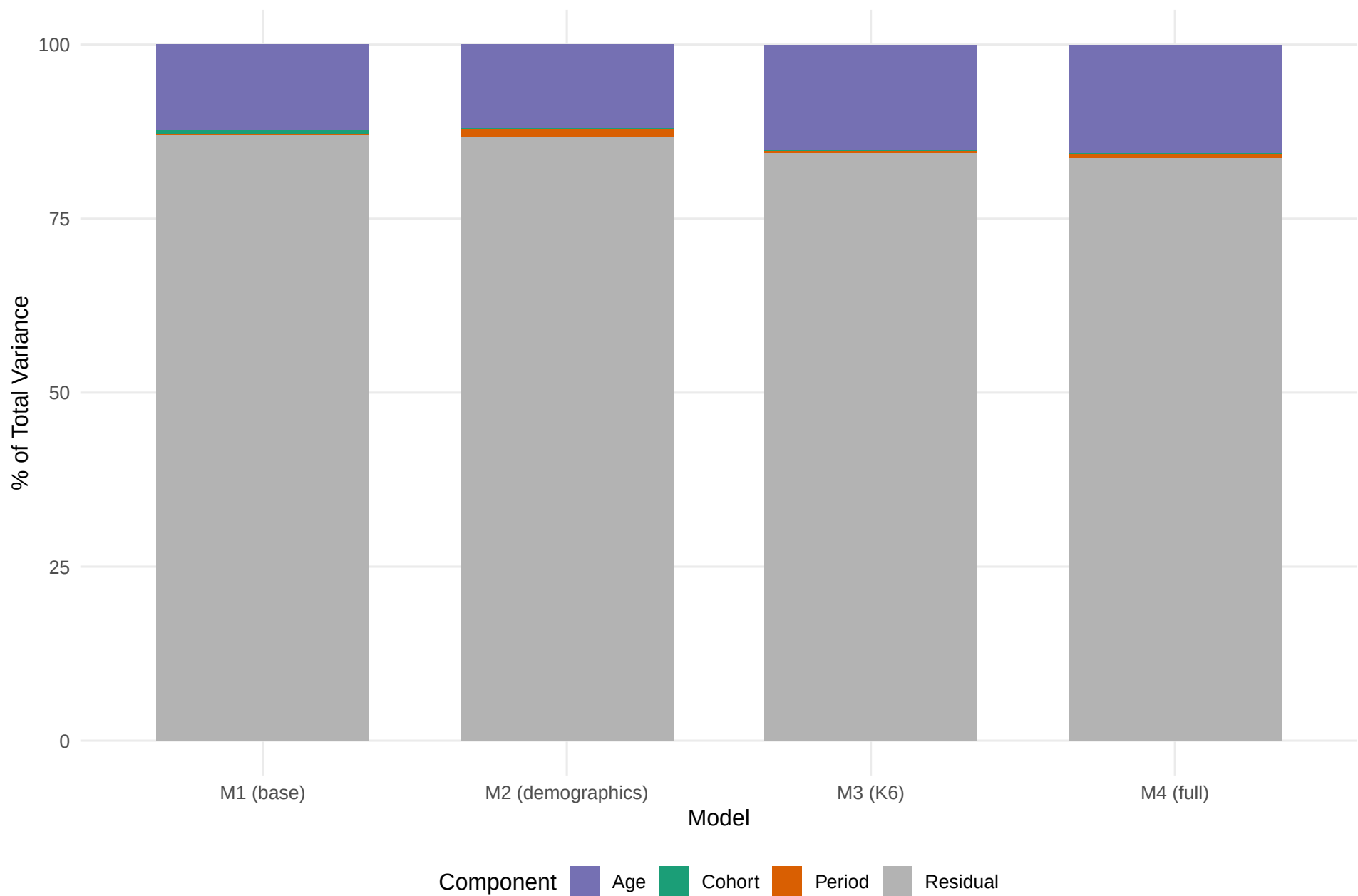
APC Variance Decomposition Across Model Specifications (NHIS)
