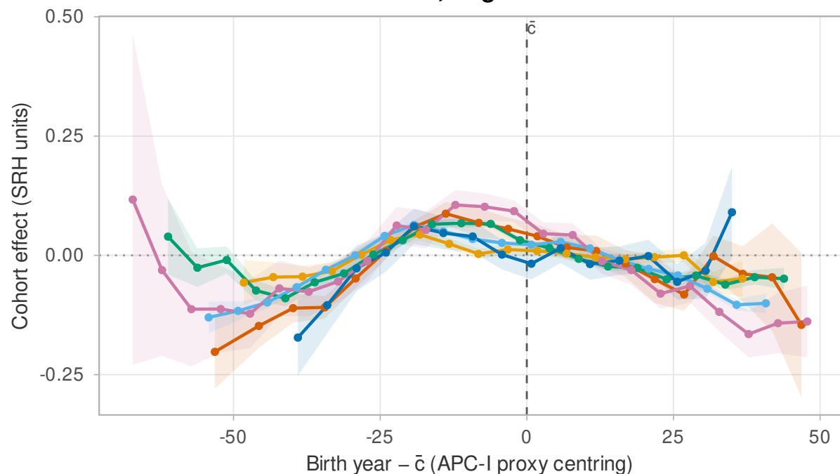
APC-I inter-cohort deviations, aligned on c - \bar{c}
