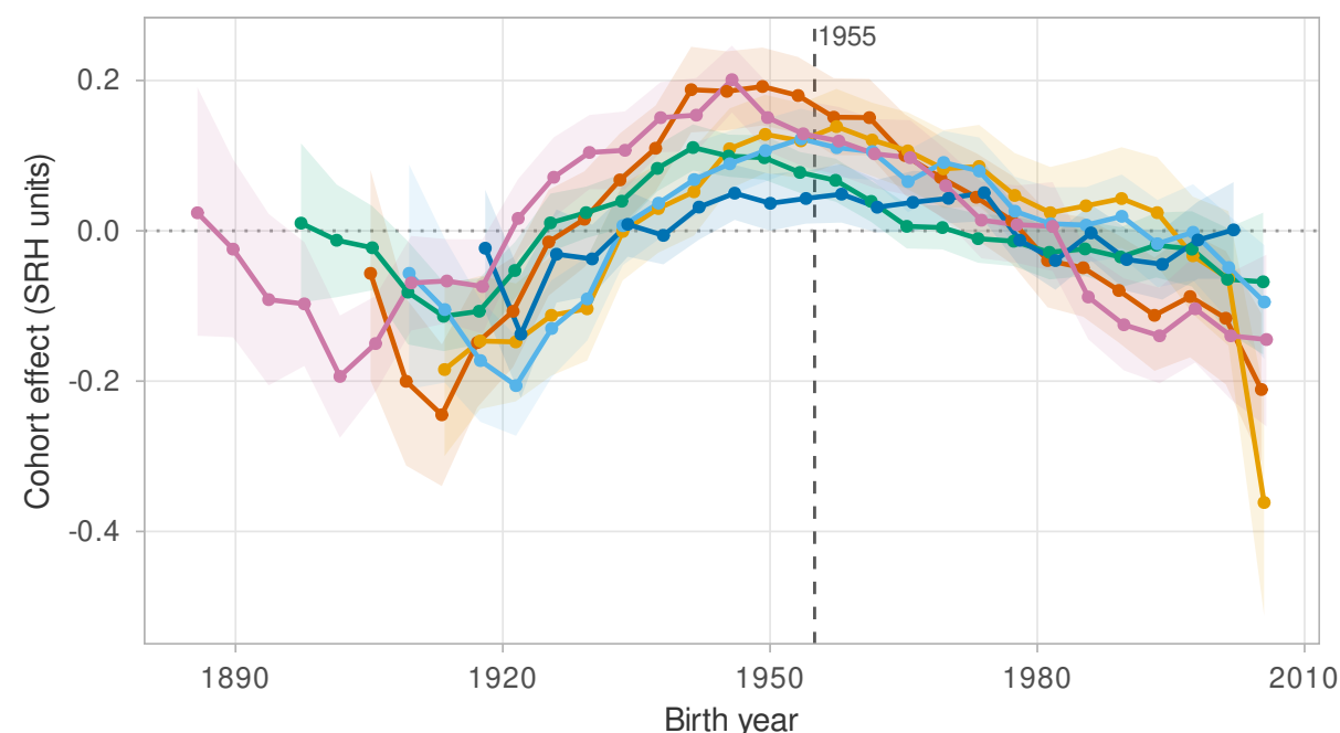
BHAPC cohort effects, raw birth year
