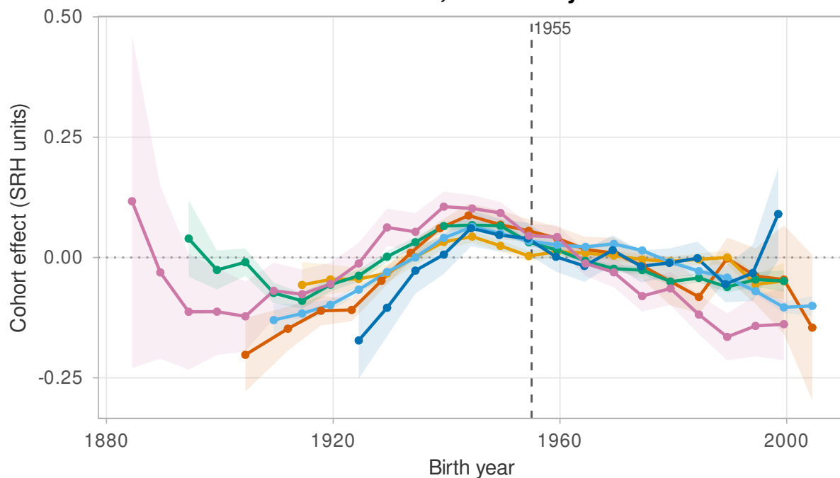
APC-I inter-cohort deviations, raw birth year
