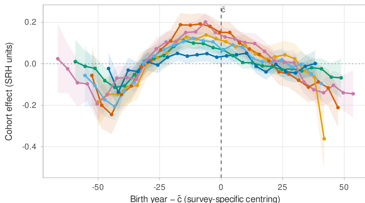
BHAPC cohort effects, aligned on c - \bar{c}
