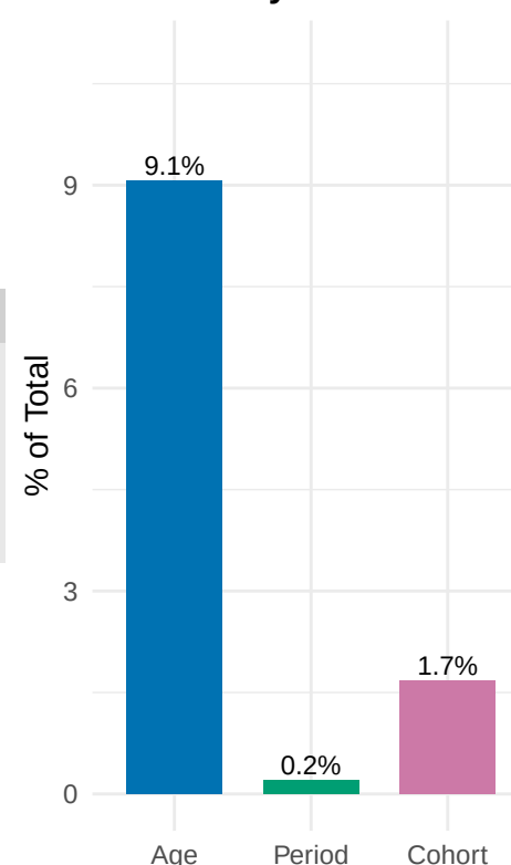
Variance by APC
