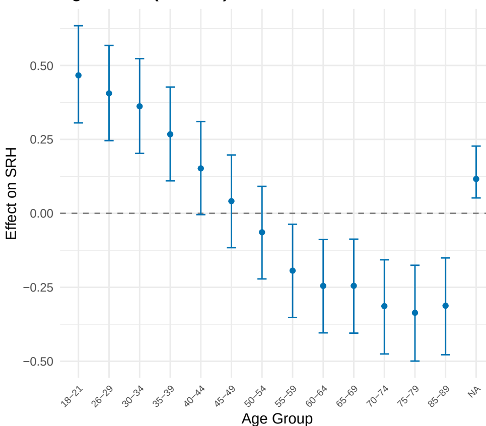
Age Effects (Random)
