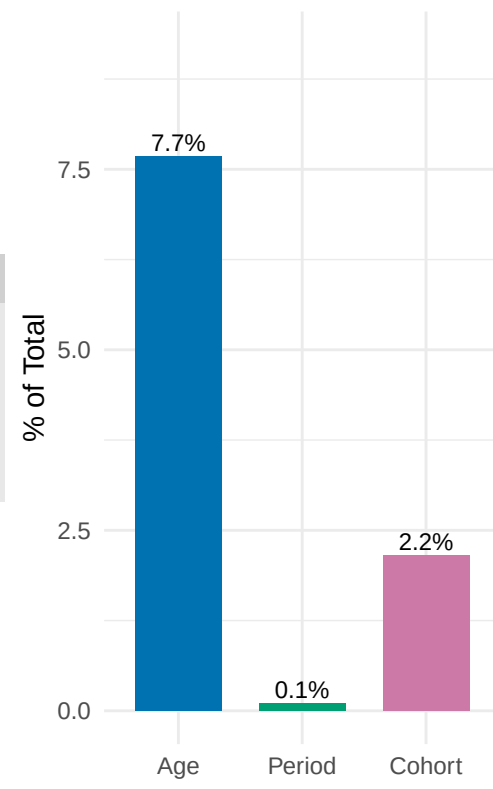
Variance by APC
