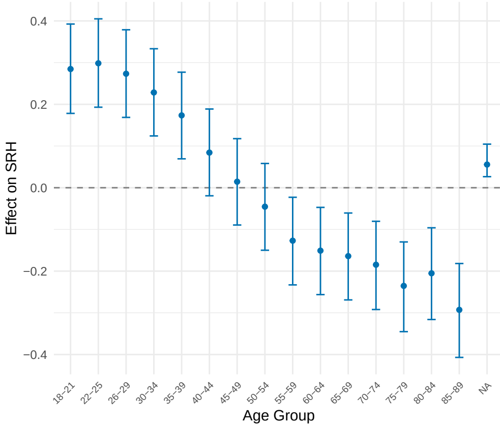
Age Effects (Random)
