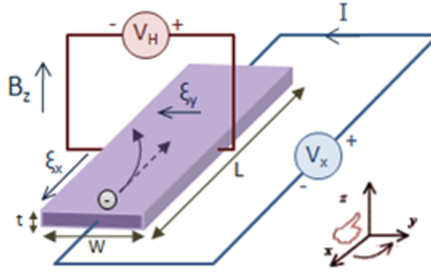
Figure 2: Hall effect
