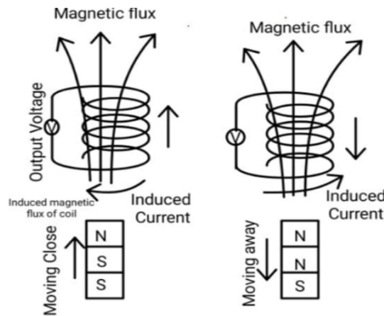
Figure 1: Lenz's law
