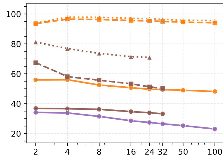
Pose AUC @ 5° ↑
