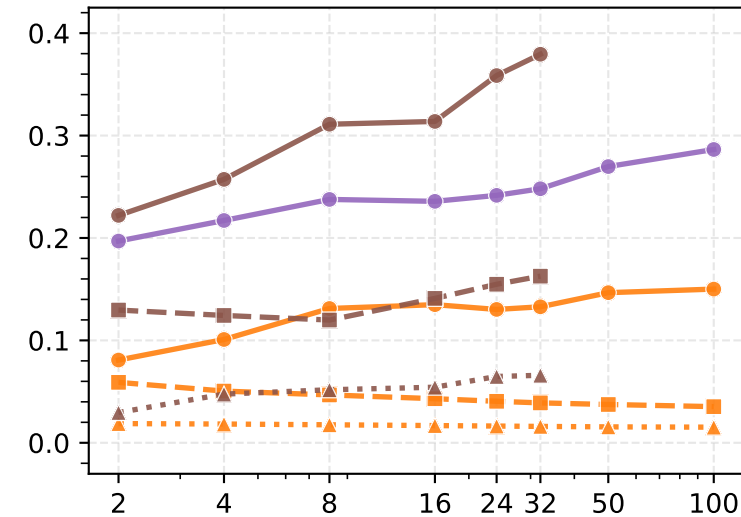
Points rel ↓
