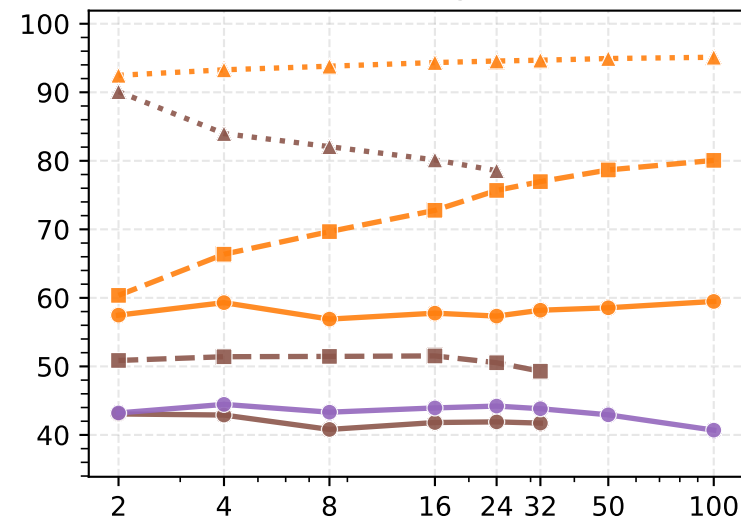
Points Inliers @ 1.03% ↑
