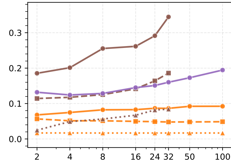
Depth rel ↓
