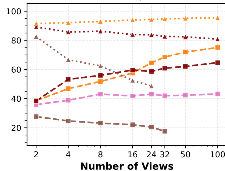
Points Inliers @ 1.03% ↑
