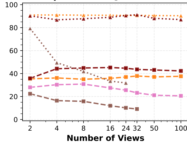
Depth Inliers @ 1.03% ↑
