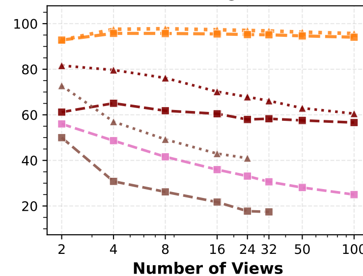
Pose AUC @ 5° ↑
