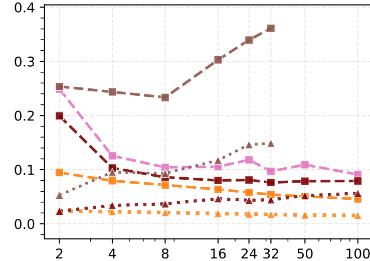
Points rel ↓
