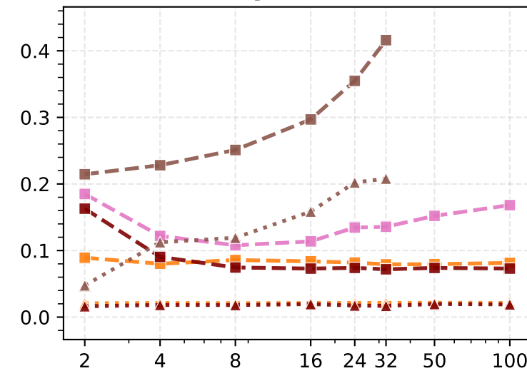
Depth rel ↓
