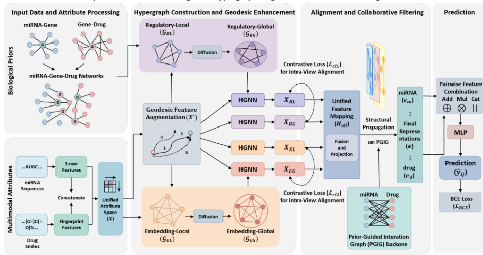
Fig. 1 Overview of GCFH-MDA.
