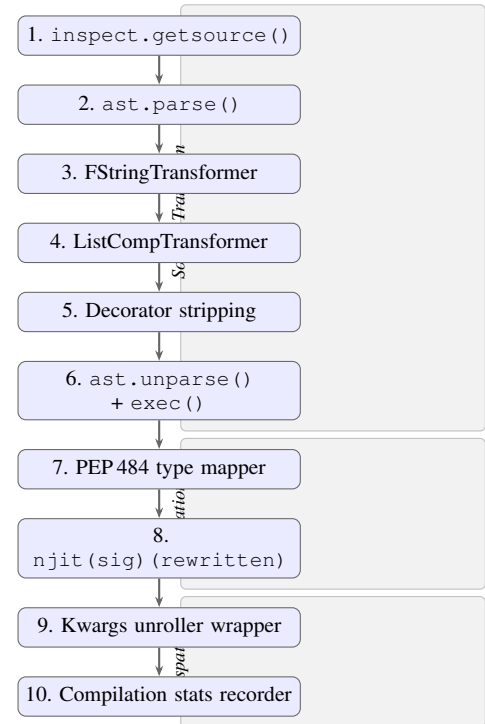
Fig. 1. The CloudSealed Compiler pipeline. All stages execute once at decoration time except stage 9, which executes per call only when keyword arguments are present.
