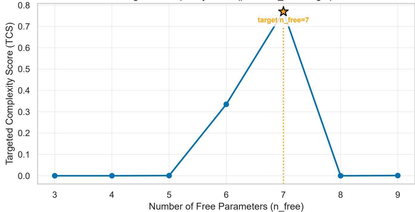
Targeted Complexity Score (prefers n_{\text{free}} \approx \text{target} )
