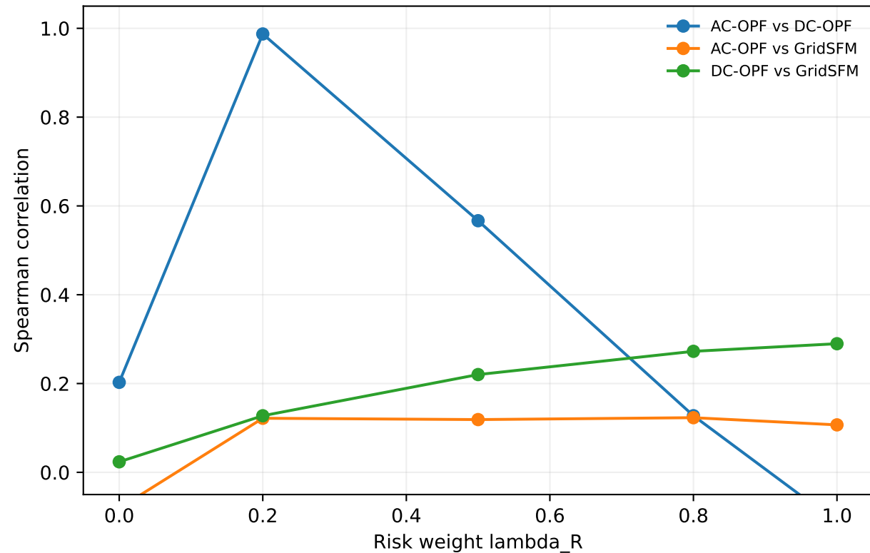
Shared K=1 rank agreement
