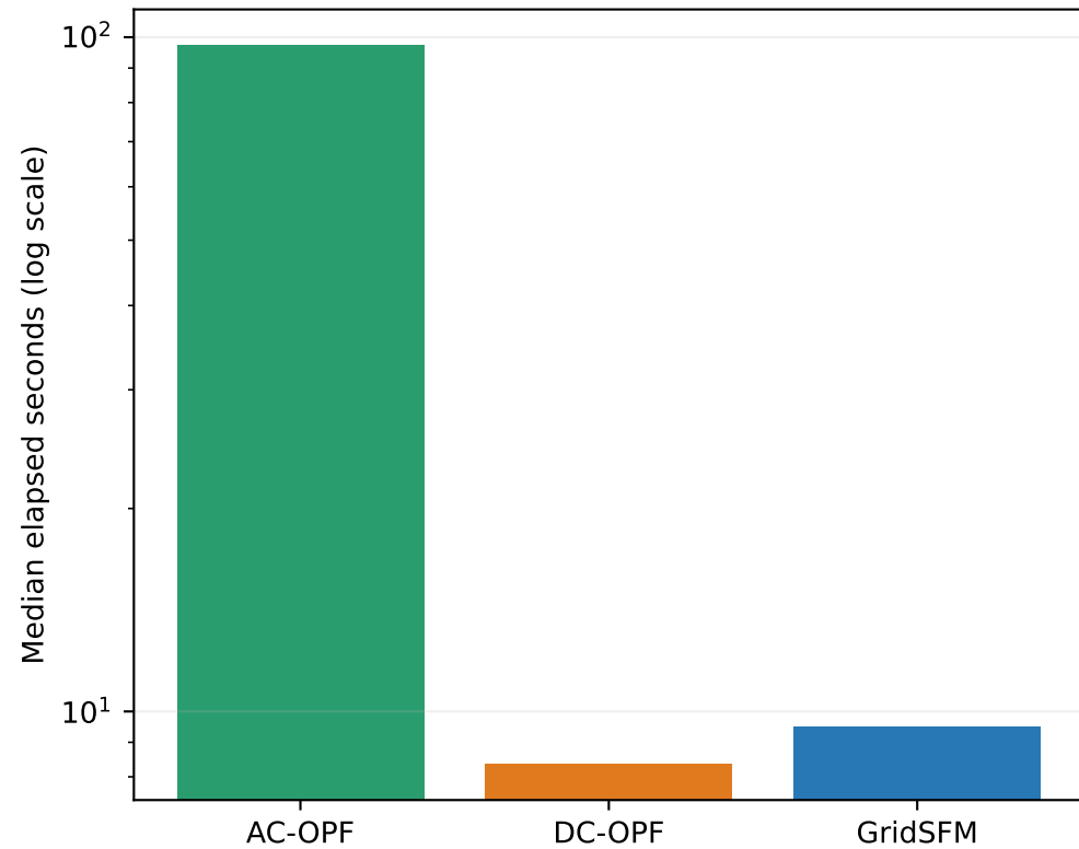
Per-candidate runtime
