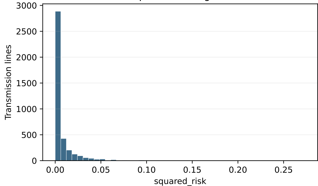
Squared-loading risk
