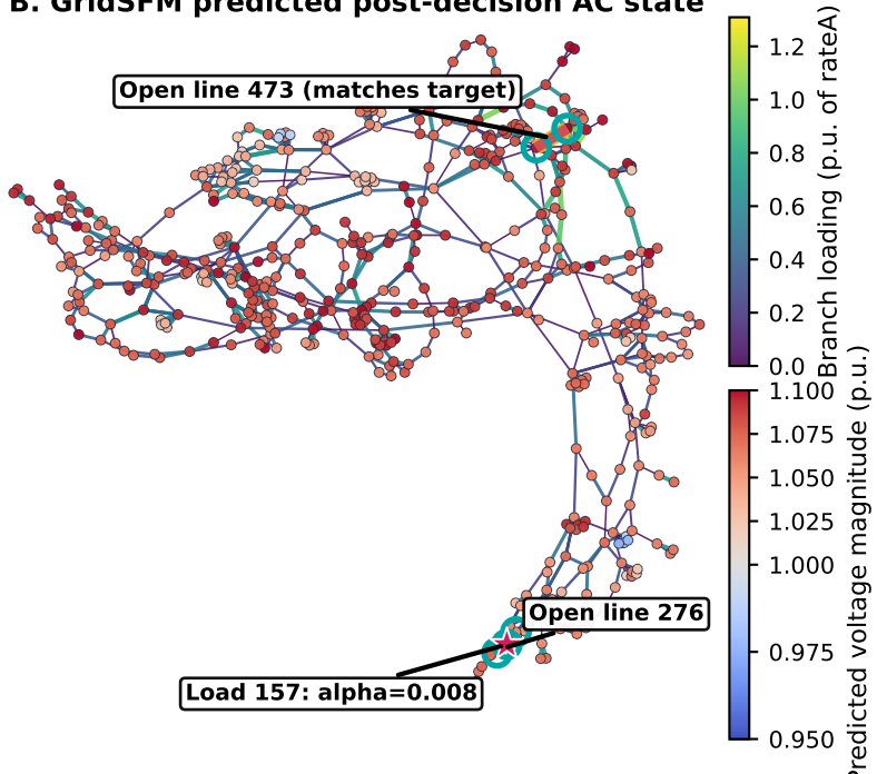
B. GridSFM predicted post-decision AC state
