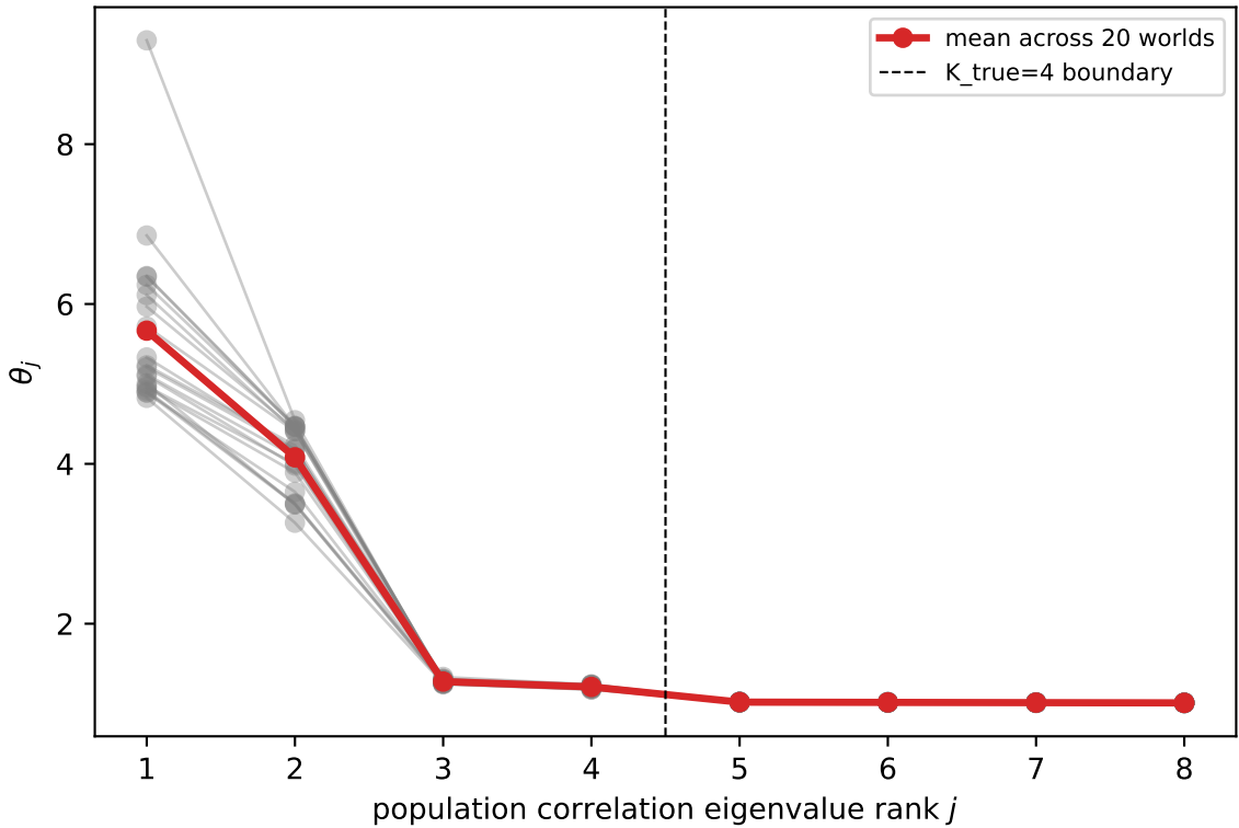
Population leading-eigenvalue profile (Lyapunov-solved stationary correlation)
