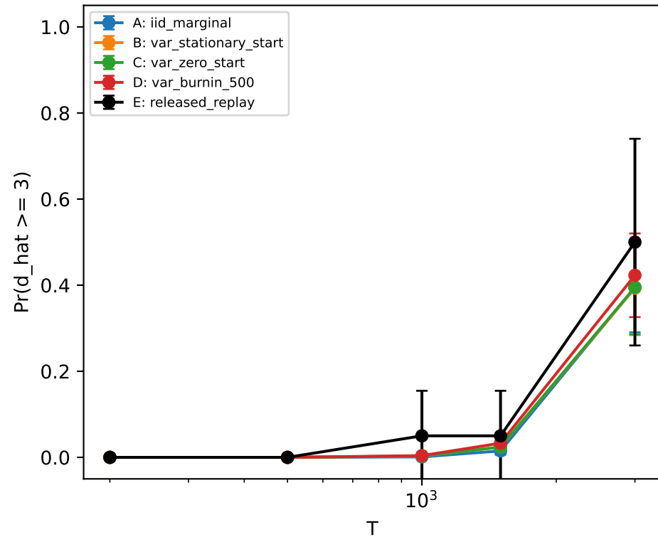
Pr( \hat{d} \geq 3 ) vs T, by branch
