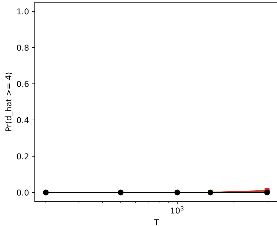
Pr( \hat{d} \geq 4 ) vs T, by branch
