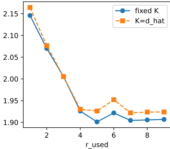
formal MSPE vs r_{\text{used}}
