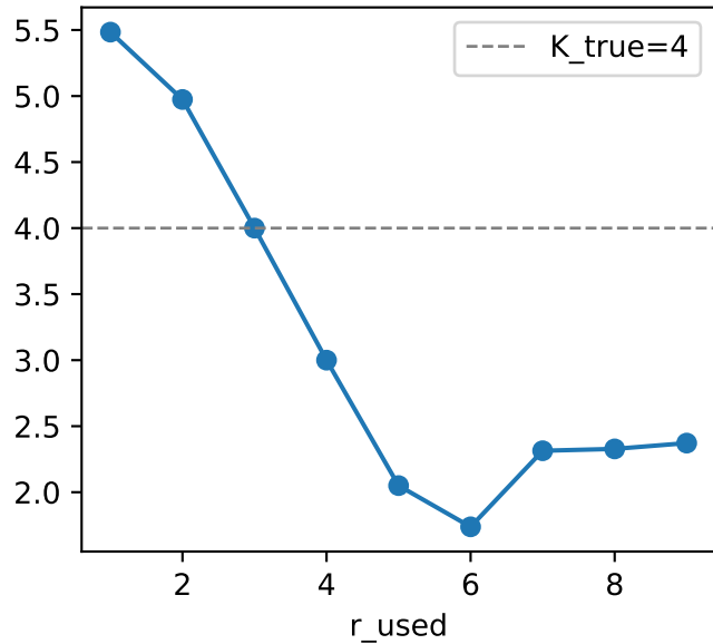
mean \hat{d} vs r_{\text{used}}
