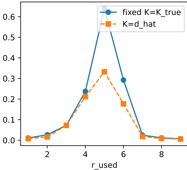
formal ARI vs r_{\text{used}}
