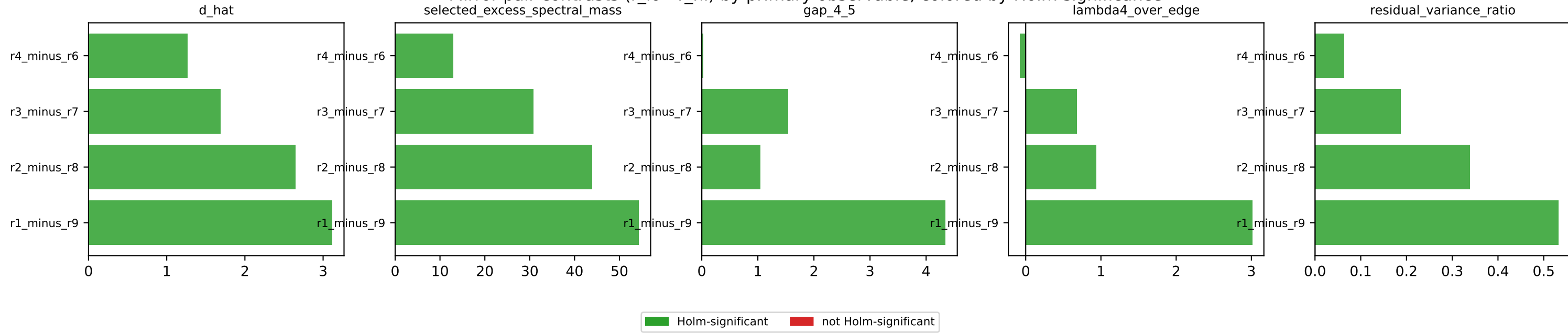
Mirror-pair contrasts ( r_{lo} - r_{hi} ) by primary observable, colored by Holm significance
