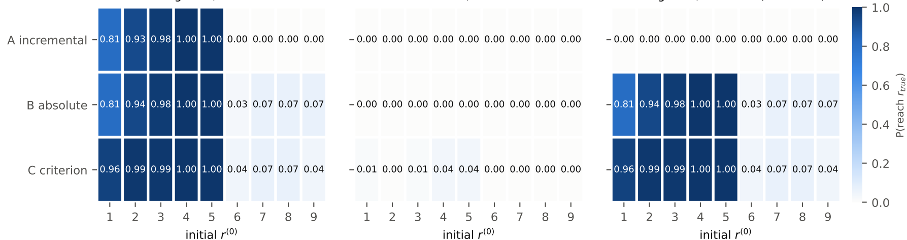
strong SBM, zero-fixed
