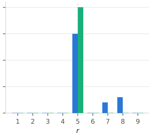
controlled diagnostic ( K = K_{true} )
